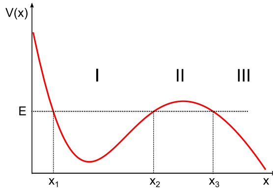
Figure 4.4: Tunneling barrier for the tilted potential. During the spilling process, atoms occupying bound states in region I can tunnel through the barrier (region II) to become free particles (region III). Both the energy levels of the bound states and the tunneling time constants are calculated using the WKB method (see text).
